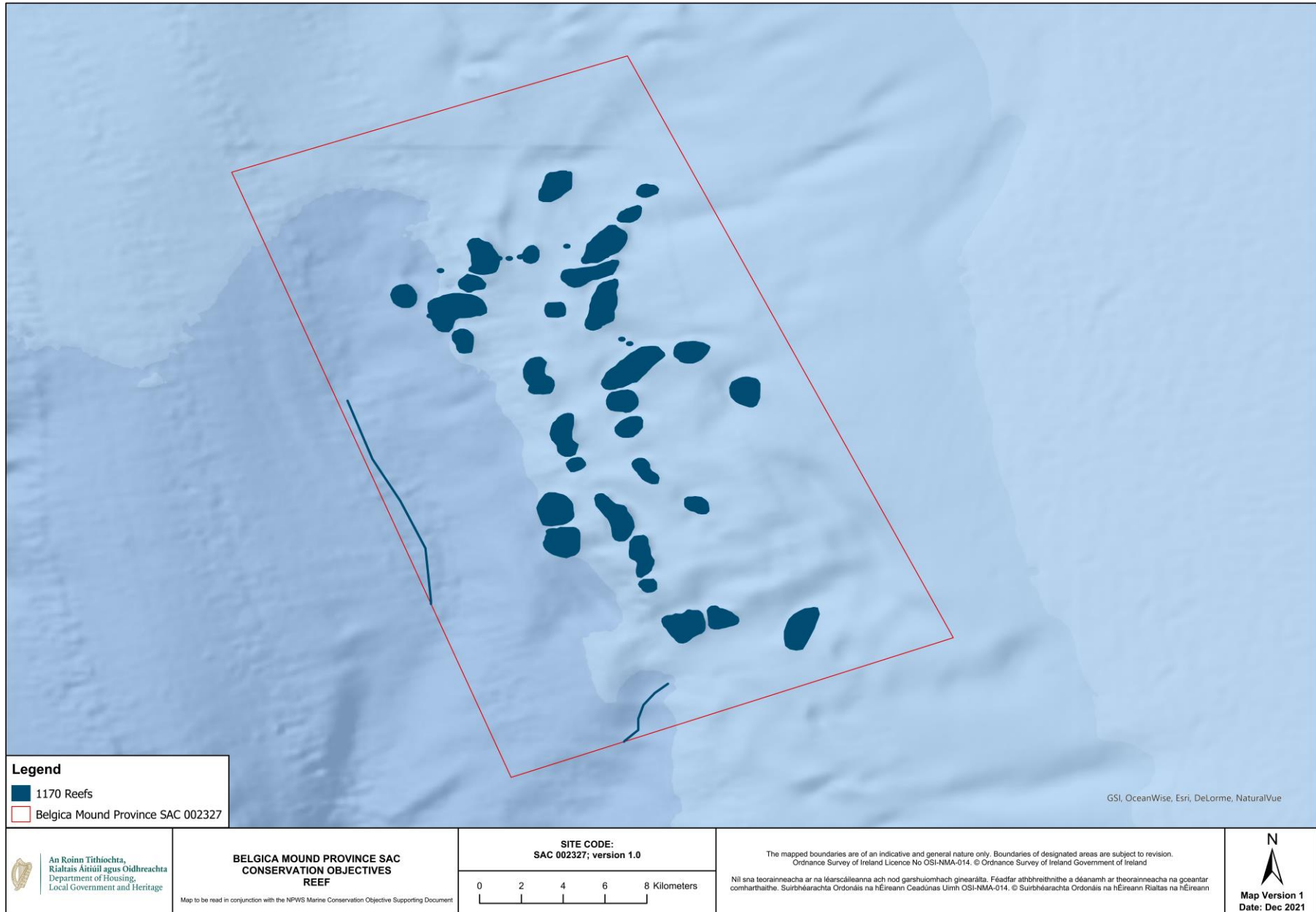
Figure 1. Mapped Annex I Reef habitat in Belgica Mound Province SAC
