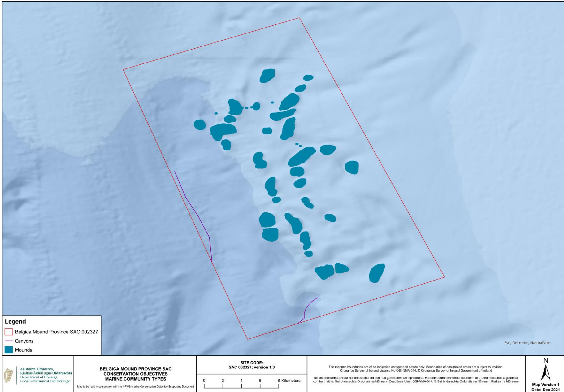
Figure 2. Mapped geological features which are used as indicators of the reef community complex in Belgica Mound Province SAC
